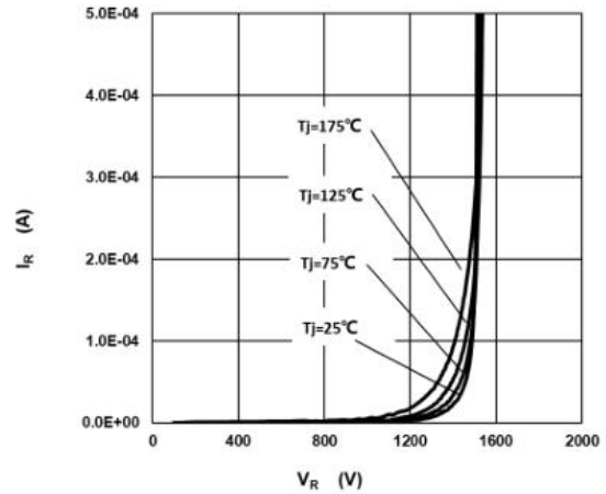
Fig.2 –Reverse Characteristics
