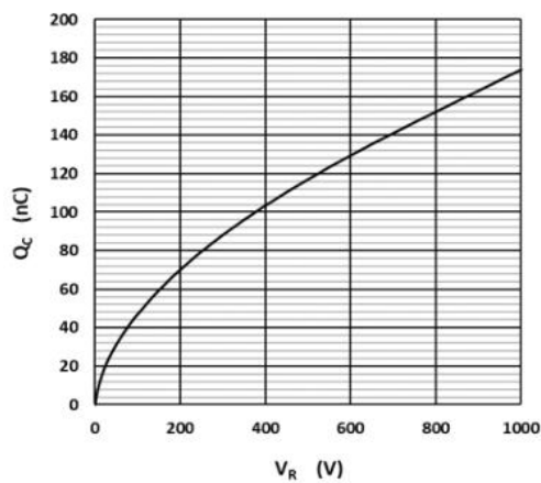
Fig.5 –Total Capacitance Charge vs. Reverse Voltage
