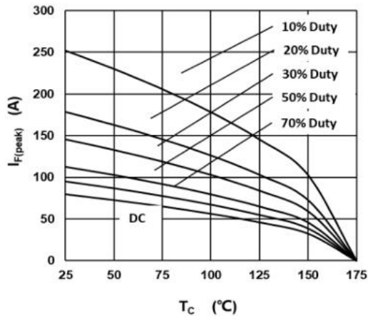
Fig.3 –Current Derating
