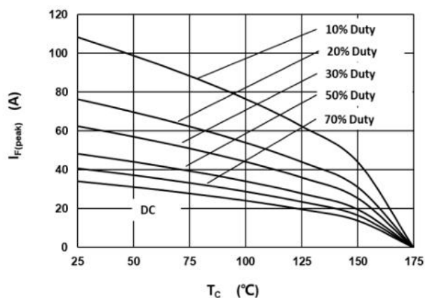
Fig.3 –Current Derating
